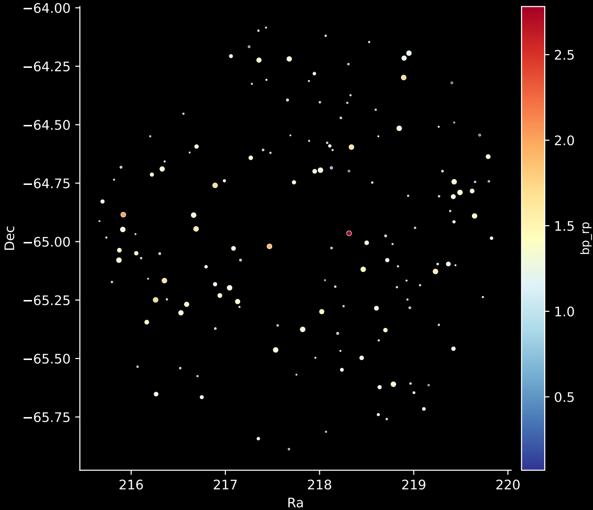
APOGEE DR17 Field: [277-18-O_TESS] Stars: 152
