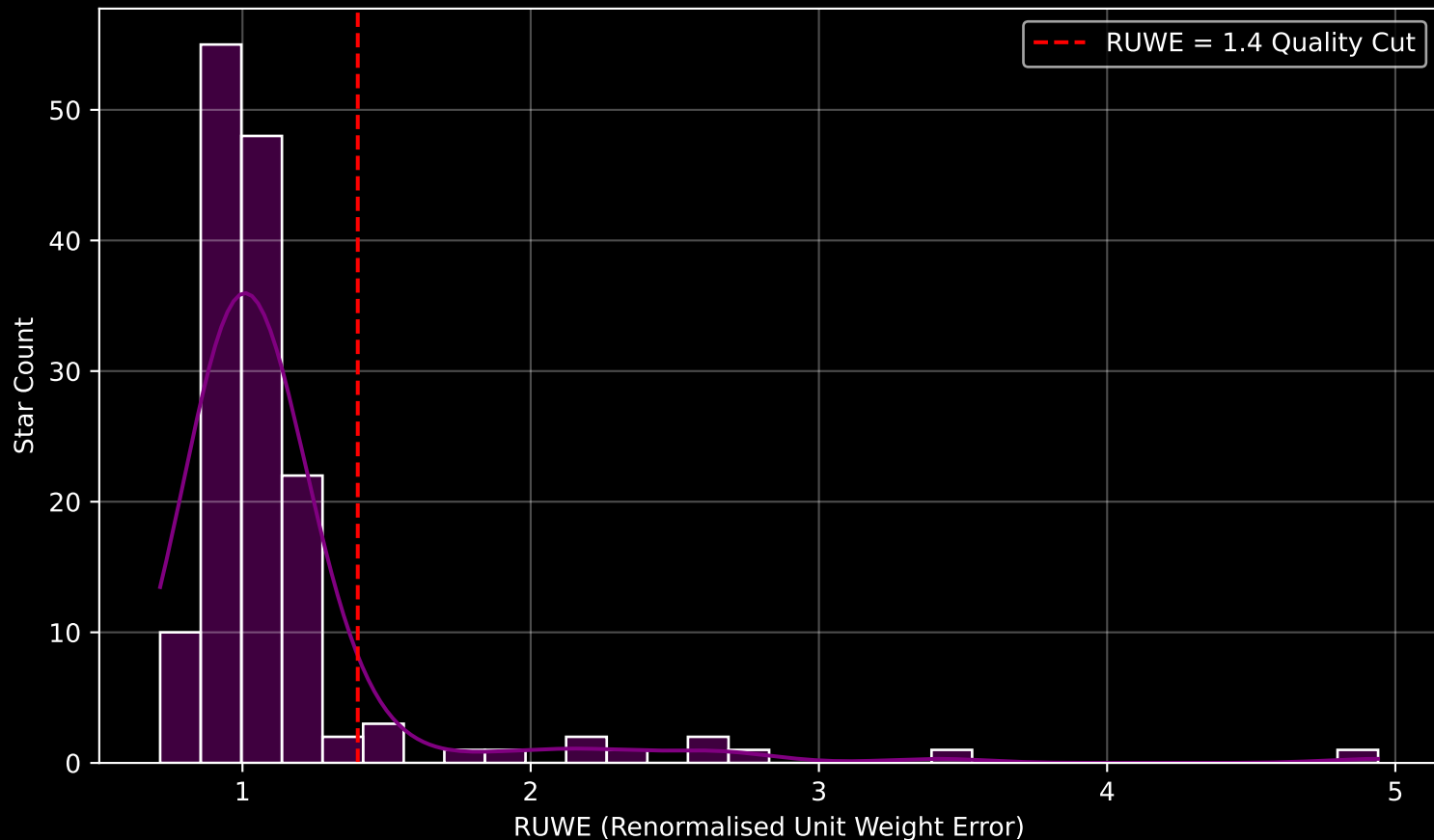
GAPOGEE DR17 Field [277-18-O_TESS] RUWE Distribution (n= 150)
