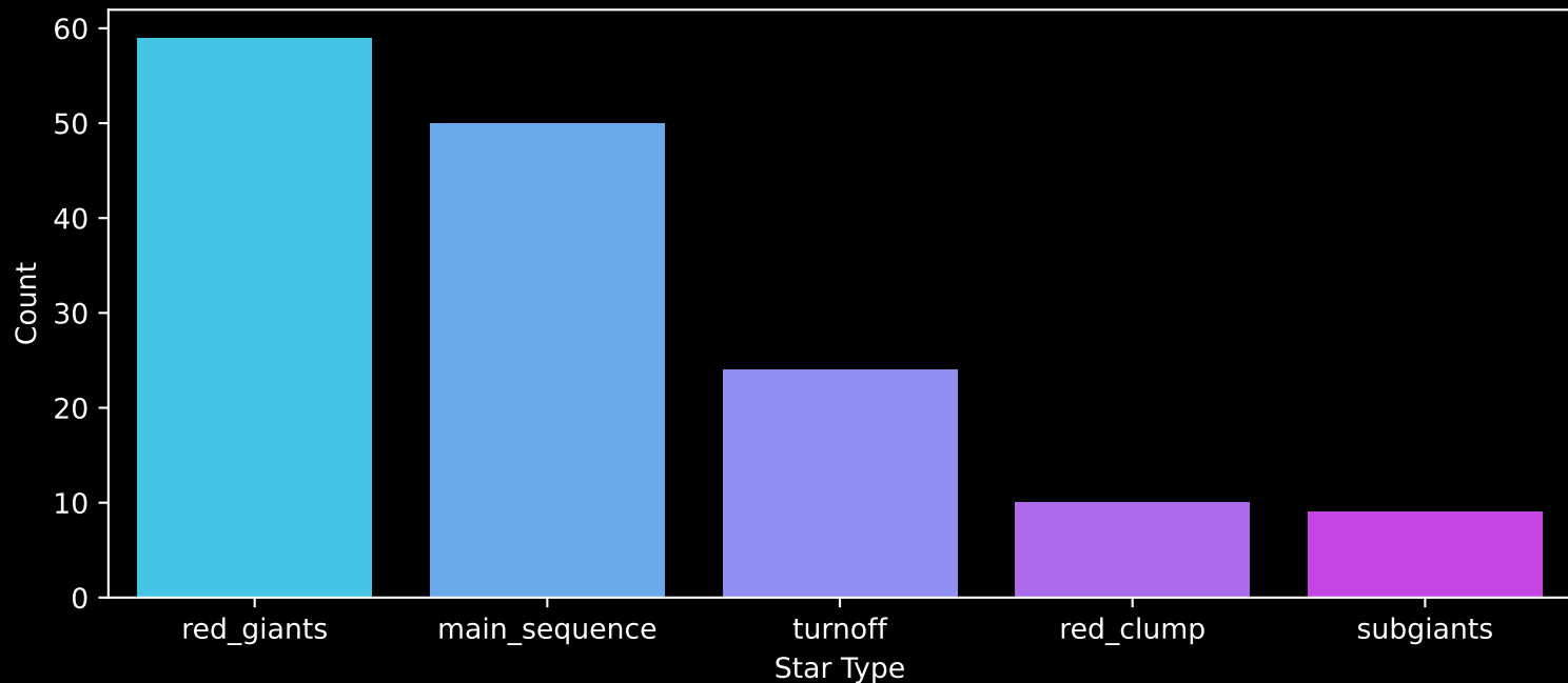
APOGEE DR17 Field: [277-18-O_TESS] Count plot of Star Type
