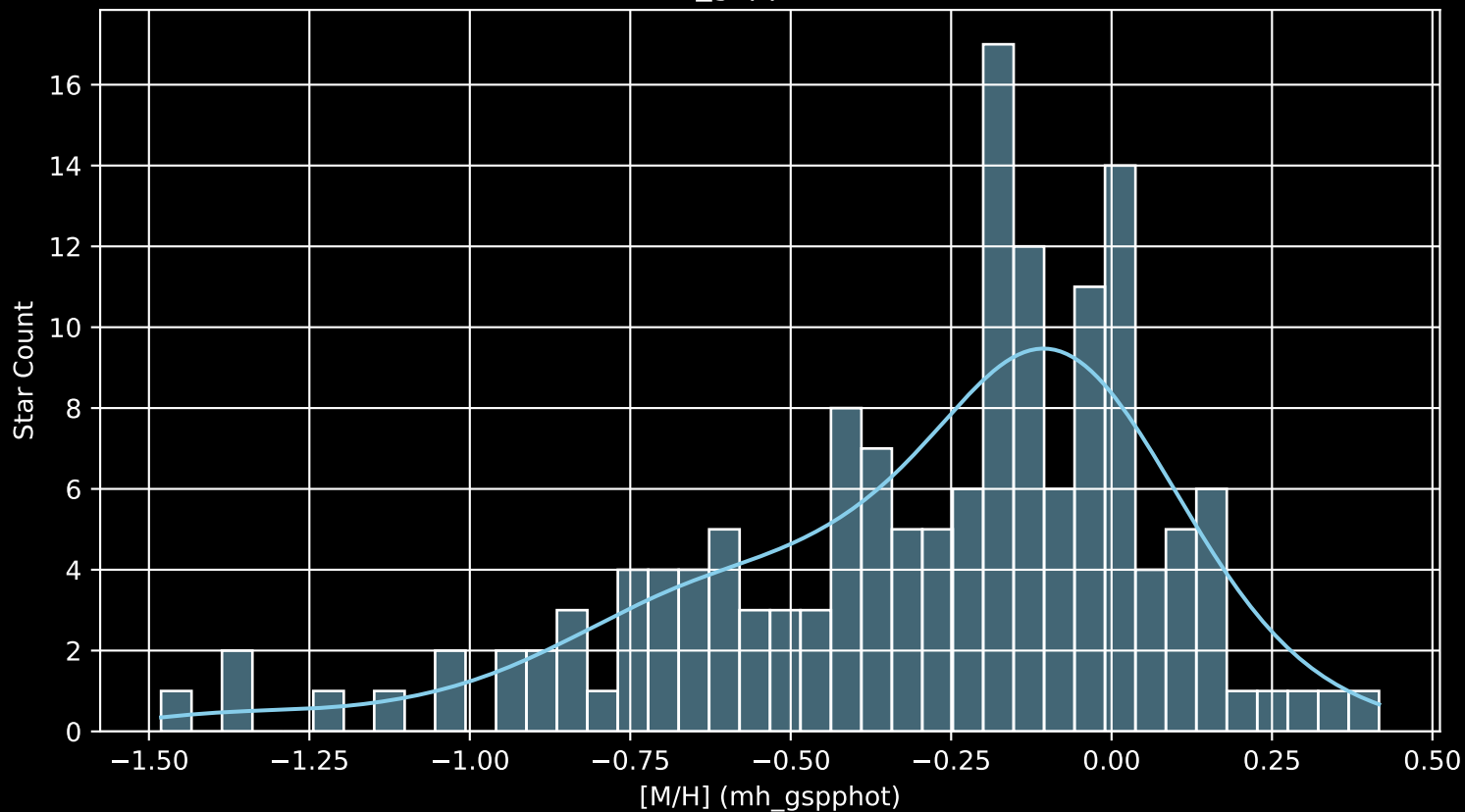
APOGEE DR17 Field: [277-18-O_TESS [M/H] (mh_gspphot) (n= 152)
