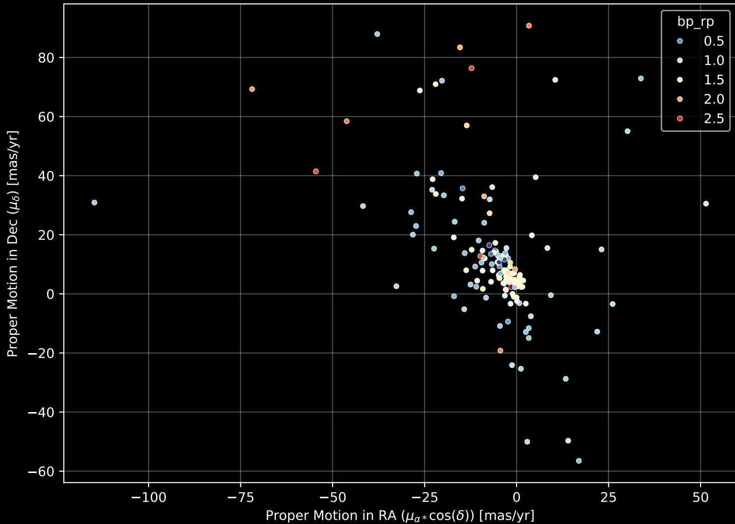
APOGEE DR17 Field: [277-18-O_TESS] Proper Motion Diagram (n= 152)
