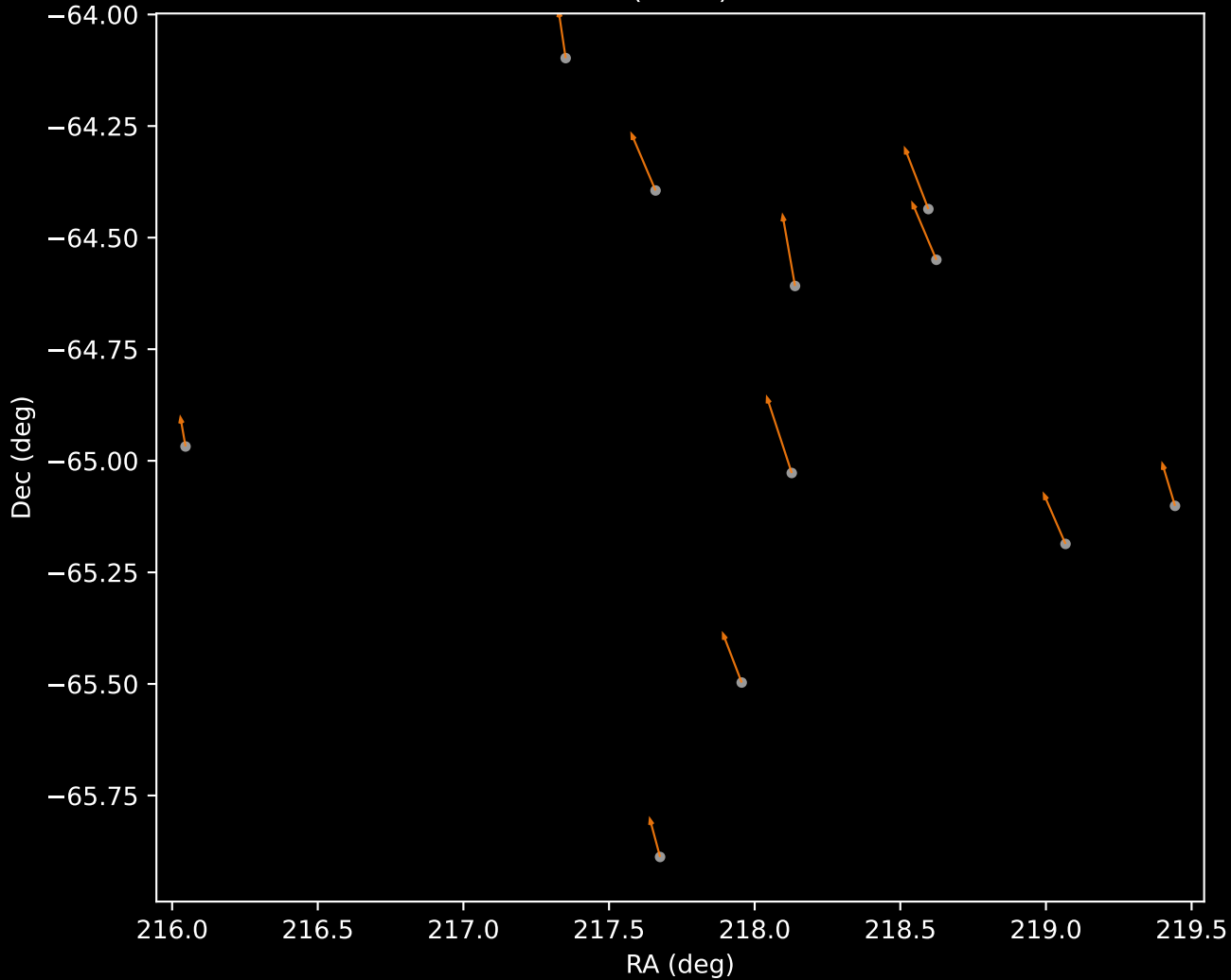
APOGEE DR17 Cluster 2 Proper Motion Vectors (n=11)
