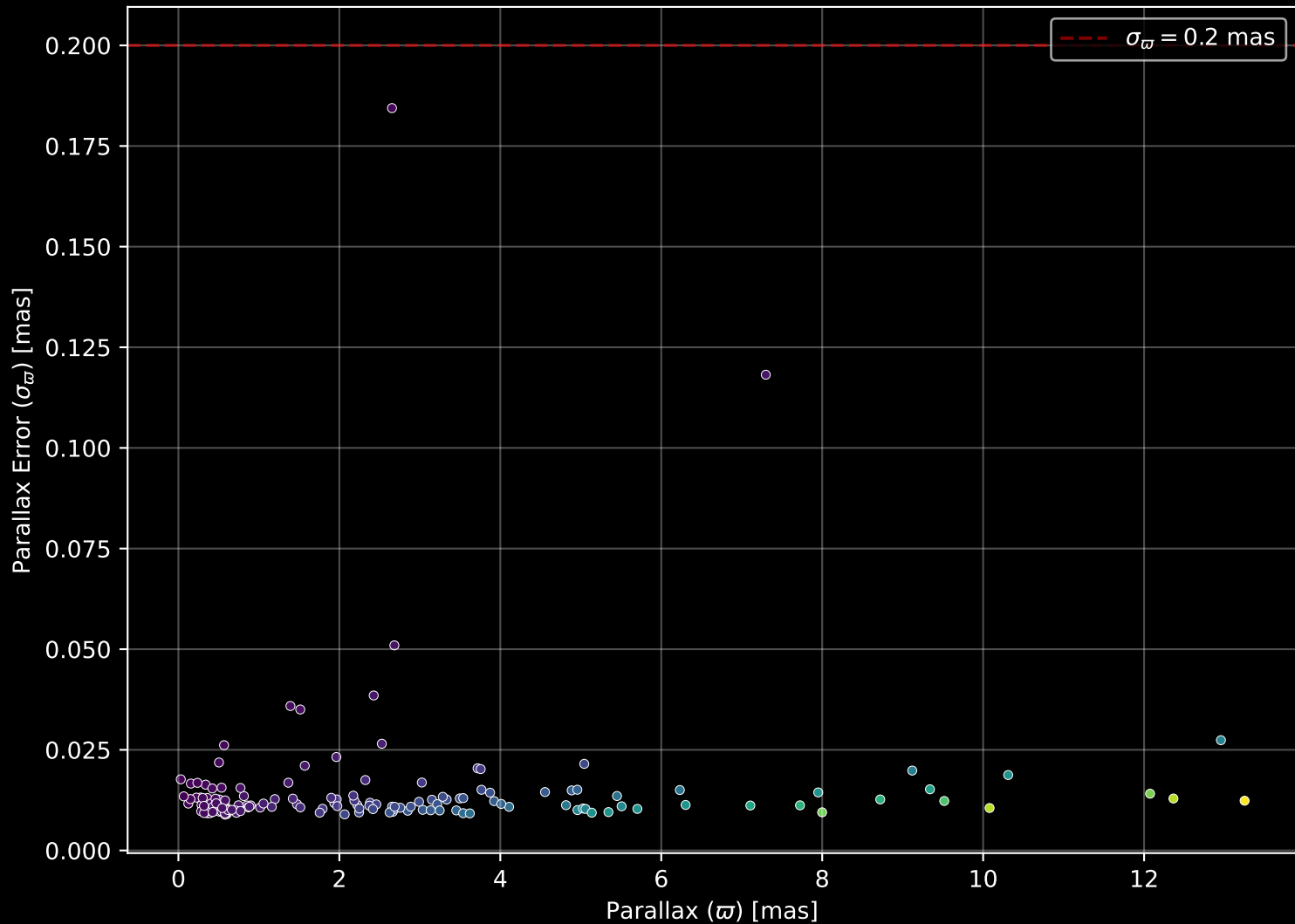
APOGEE DR17 Field: [277-18-O_TESS] Parallax Quality (n= 152)
